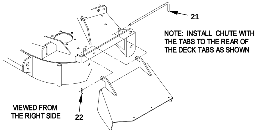
FIGURE 9 DISCHARGE CHUTE INSTALLATION
