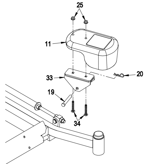
FIGURE 8 REMOVABLE WEGHT INSTALLATION
