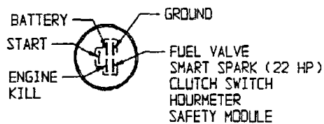
IGNITION SWITCH
